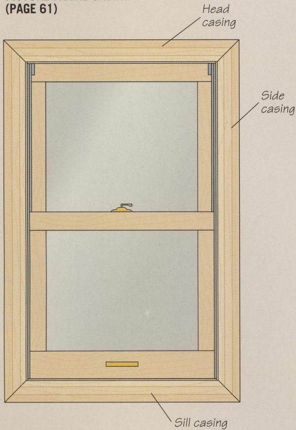
STOOL-AND-APRON CASING (PAGE 69)
