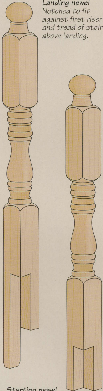
Starting newel Extends to floor at bottom of stairs; notched to fit around open-stringer end of bottom riser and tread. Could be made longer to extend through sub-floor and be bolted to floor joist for added support
