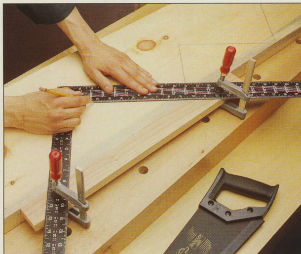
A simple jig consisting of a 1-by-4 clamped to a carpenter's square is used to mark the rise-and-run—the width of the treads and risers—on a staircase stringer.
