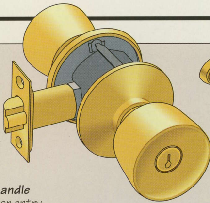
Entry lockset Features bell handles and a keyed entry lock
