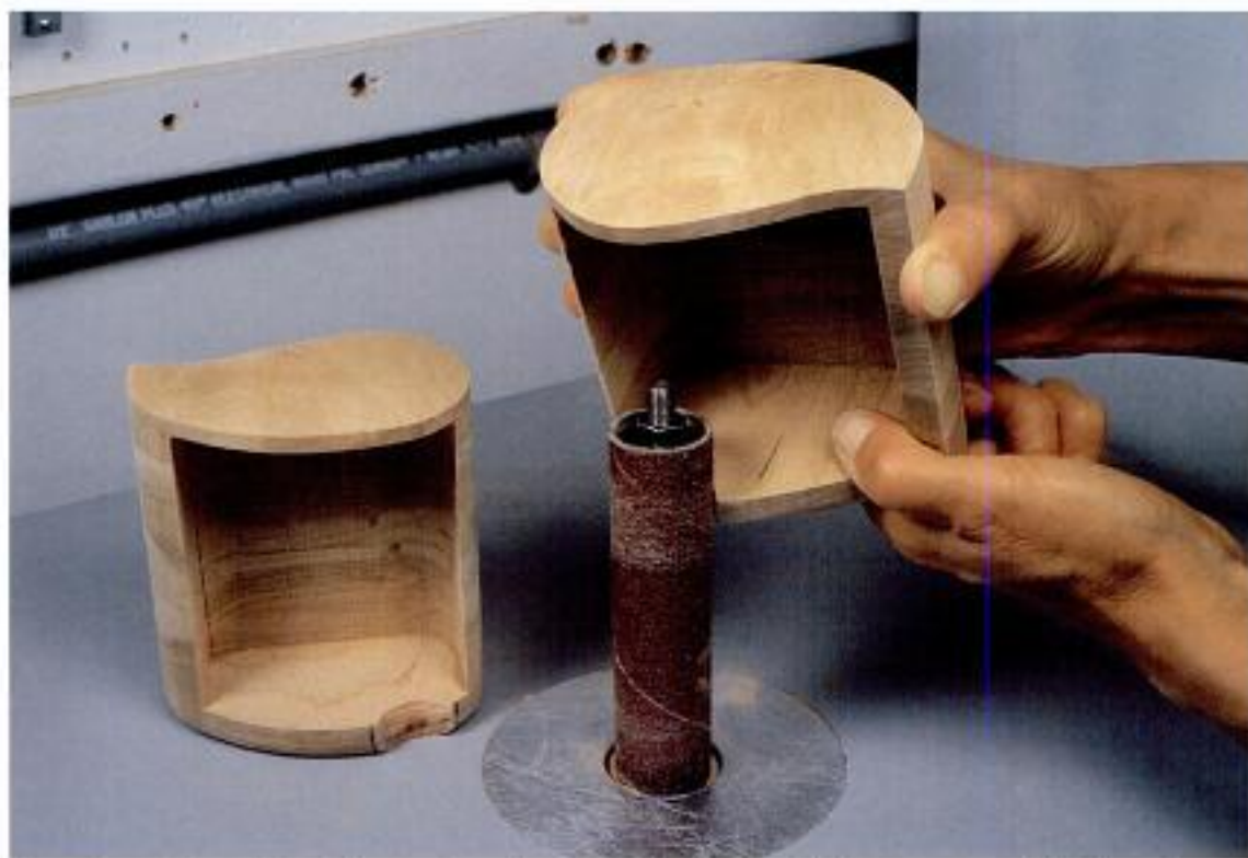
Photo 4-23 The oscillating drum sander, with a coarse sleeve on the 1" drum, can start off the finger slots.
