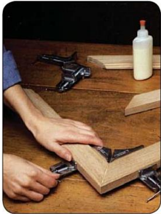
A corner clamp holds the adjoining pieces of a miter joint at 90^\circ . Applied on each of the corners of a picture frame, these clamps will produce a perfectly square frame.
