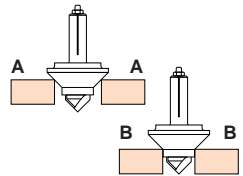
Diagram showing rise and fall of the cutter as it travels along the slot
