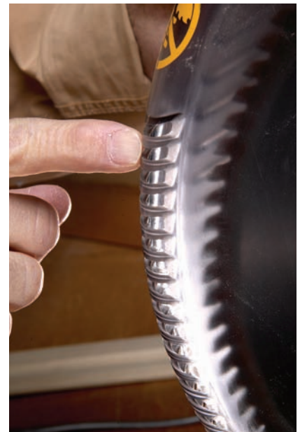
Slots are superior. Some blade guards get dusty or distort the location of the spinning blade. I prefer guards that have open slots so you can get a clear picture of where the blade is.
