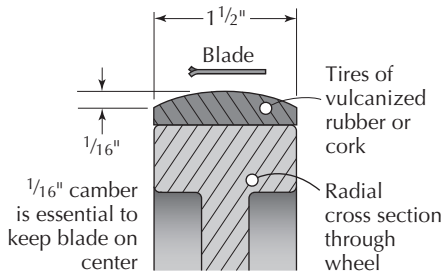
Essential camber. Band saw tires are typically cambered. If you're having trouble keeping your blade on track, you might investigate your tires.
