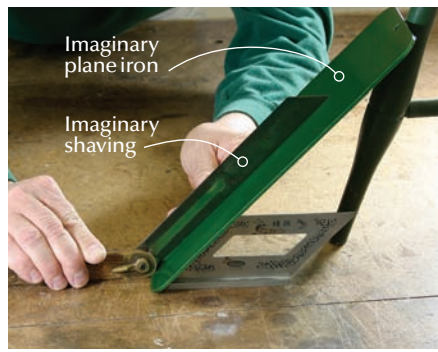
On the diagonal. As you can see in these pictures, moving slightly at a diagonal across a surface actually presents a lower angle of attack, and helps prevent tear-out.
