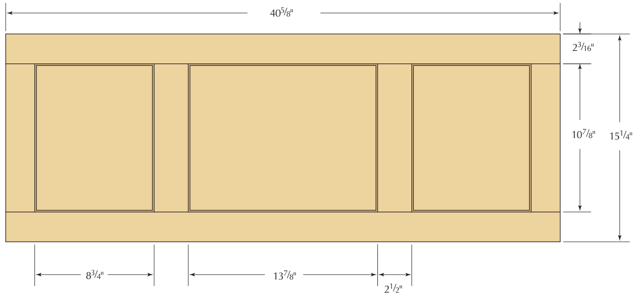
Bottom Panel Detail
