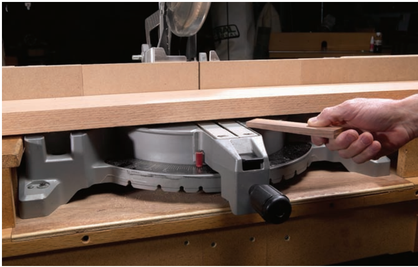
Shims make it safer. If a rough board won't sit flat on the table of your miter saw, you should shim it from below to prevent it from rocking during the cut.
