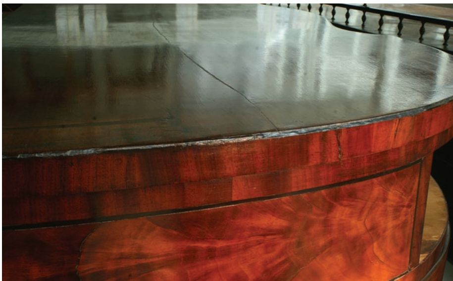
Immovable object. This solid mahogany sideboard top is badly split. The top itself is only about \frac{1}{4} " thick, but it is set on an inflexible substrate: a rail-and-stile structure. The top moved but the substrate did not, so it split.
