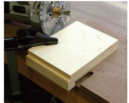
Best router setup. A platform jig, \frac{3}{4} "-dovetail router bit and a \frac{3}{4} "-outside-diameter guide bushing are used to create the sliding dovetails that attach the drawer blades to the case. It's simple.
