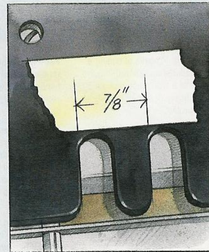
Measure finger width on dovetail template.
