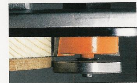
Interchangeable bearings of varying diameter control the cutting width of rabbeting bits.
