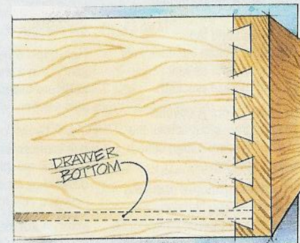
Size parts to get half tails at top and bottom.
