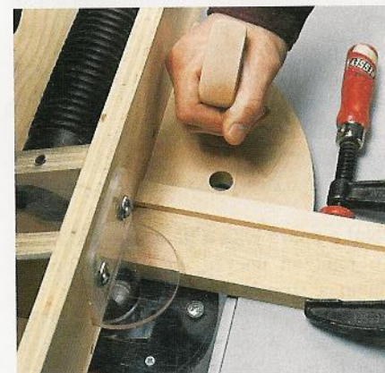
A shop-built pushblock helps move the workpiece past the built to rout end grain. Clamping the workpiece to a push block keeps it square to the fence.
