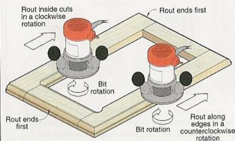
Handheld operation
