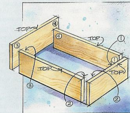
Mark edges and inside corners of each drawer.
