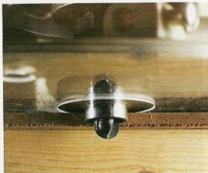
This handheld router equipped with a shop-made auxiliary base, template guide bushing, and core-box bit is ready to tackle a template-routing task. Note that the operator is using the outside edge of the template to set bit cutting depth.
