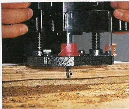
A bearing on this flush-trimming bit guides along the pattern edge, and cuts an identical edge on the piece above it. This setup is an excellent way to make finish-quality, duplicate workpieces quickly and without any additional work.
