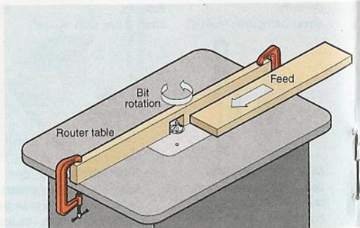
Router-table operation
