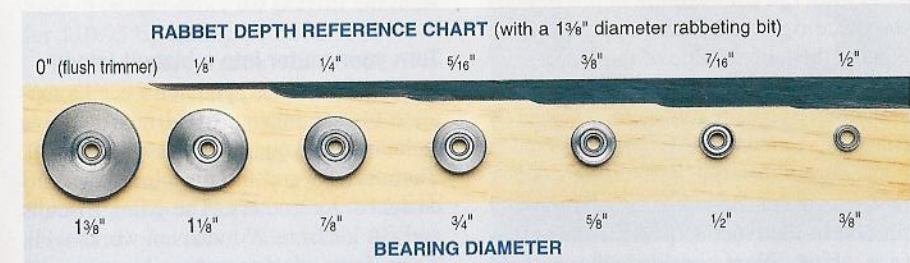
Samples of cutting depths made by different rabbeting bits and bearing combinations.
