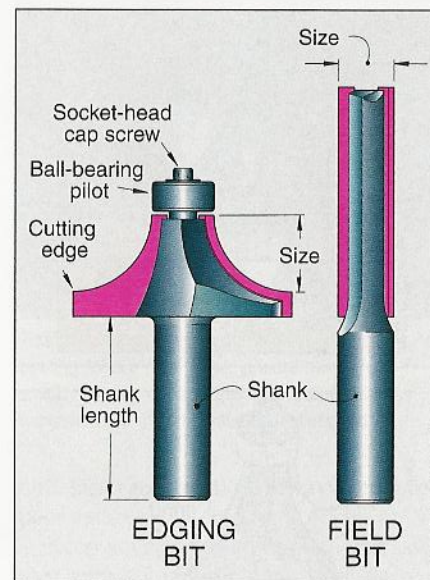
Bits have key components and dimensions that help identify them. Dimensions reference overall length; shank diameter and length; cutter length and width or diameter; and, on some bits, the cutter's angle or radius and bearing diameter.
