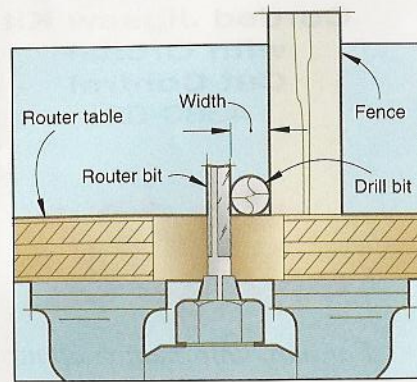
Using drill bits for quick and accurate router settings.
