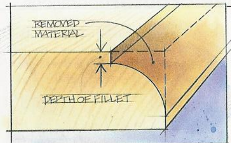
By extending a roundover bit, you can form an edge with an interesting, decorative fillet like this.
