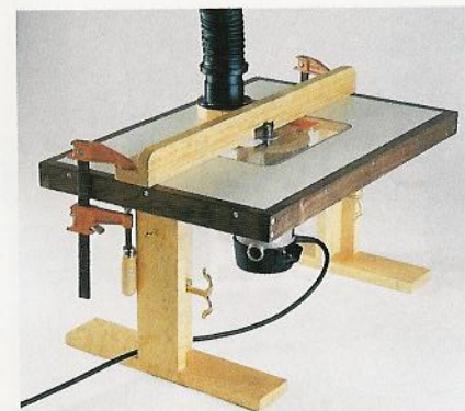
You can get the plans for building this low-cost bench-top router table. See text for information.
