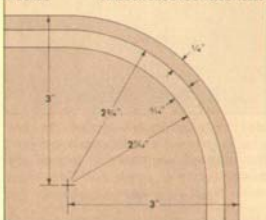
FIGURE 2 TAMBOUR GROOVE ON SIDE PIECES
