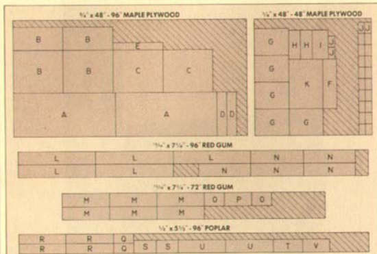
CUTTING DIAGRAM
