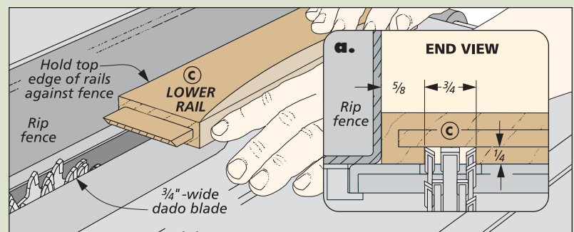
Cutting the Dadoes. The dadoes in the lower rails that hold the shelf can be cut quickly with a \frac{3}{4} "-wide dado blade installed in the table saw. Clearly mark the top edge of each rail and then hold that edge against the fence. Gradually raise the blade to sneak up on the final depth of the cut.
