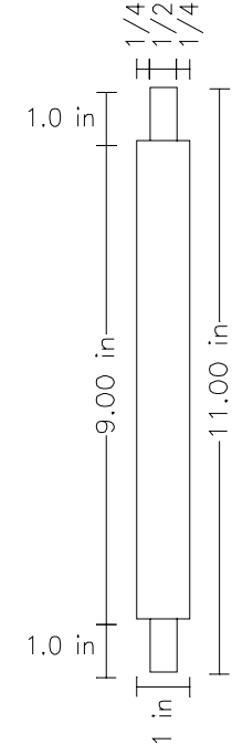
Top View
