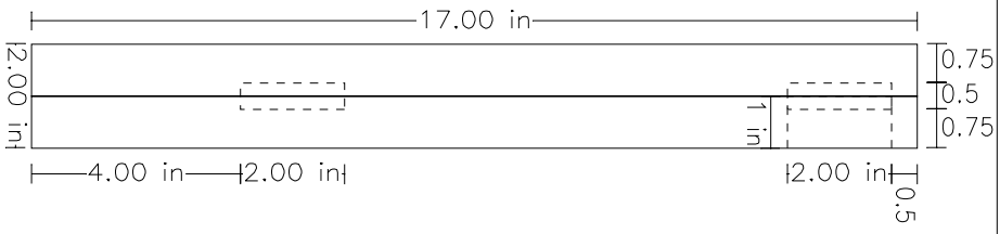
Side View
