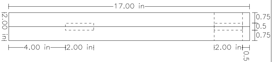
Side View
