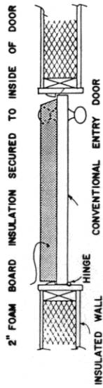
2" FOAM BOARD INSULATION SECURED TO INSIDE OF DOOR
