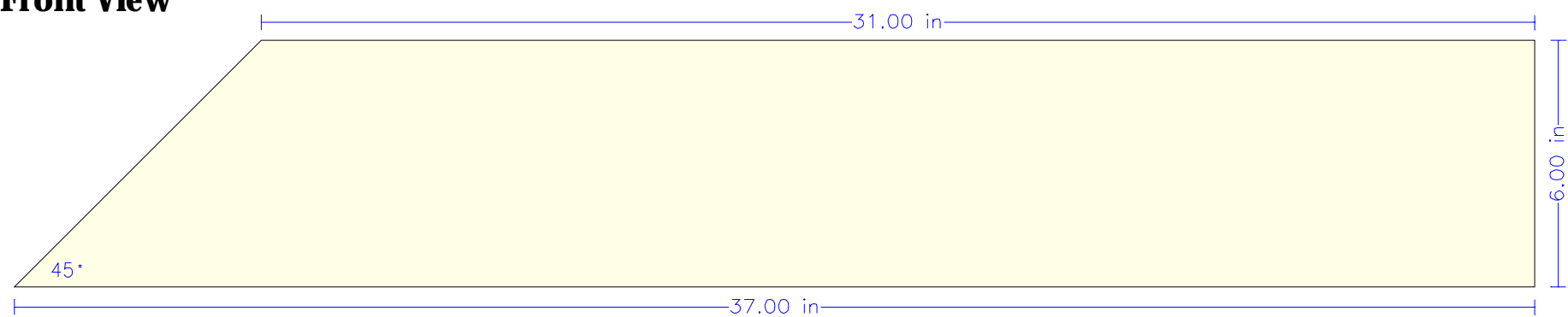
Front View
