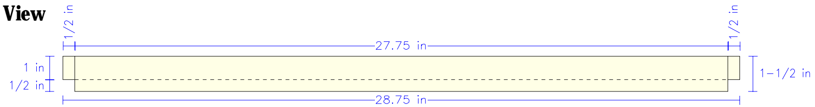
Top View
