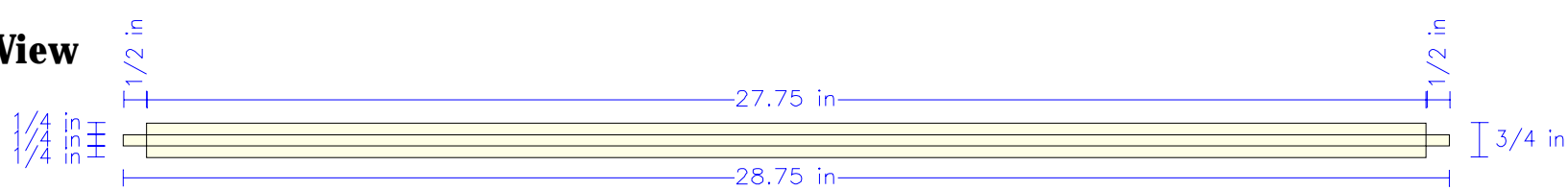
End View
