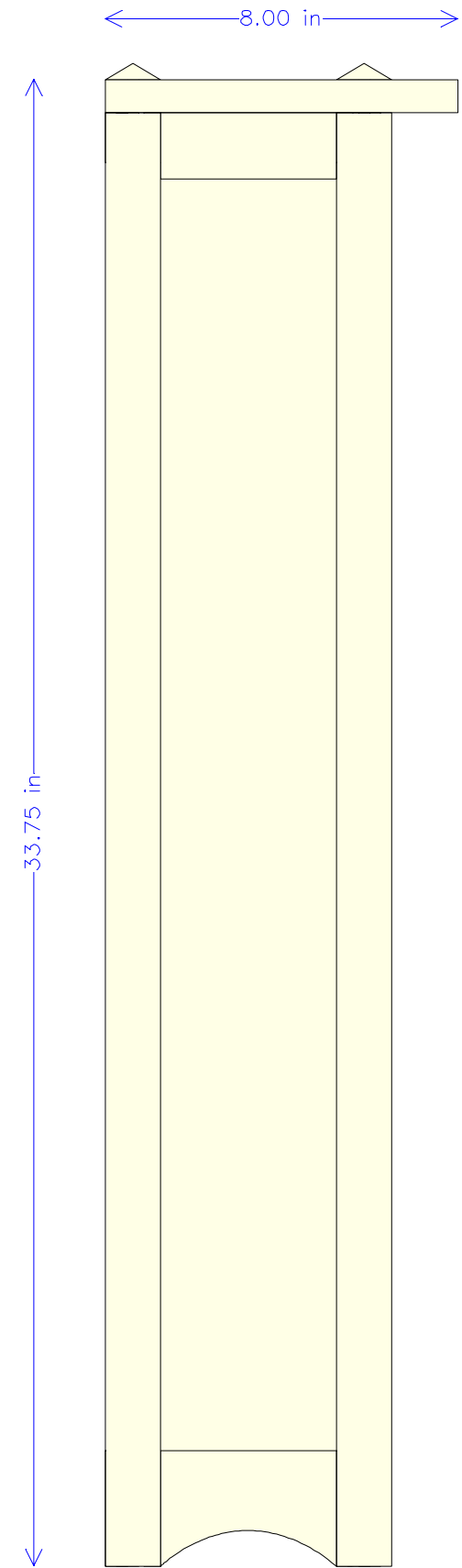
Side View
