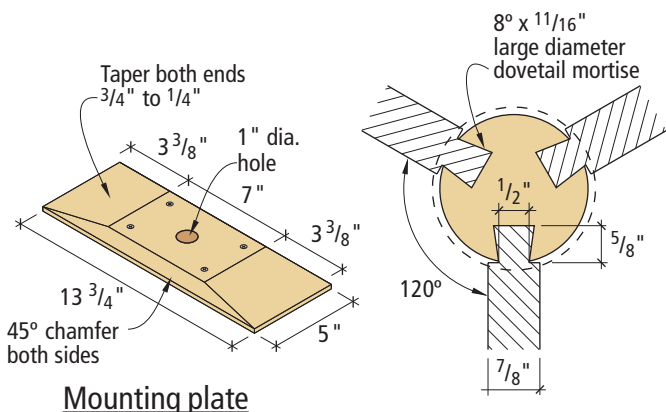
Leg to pedestal dovetails
