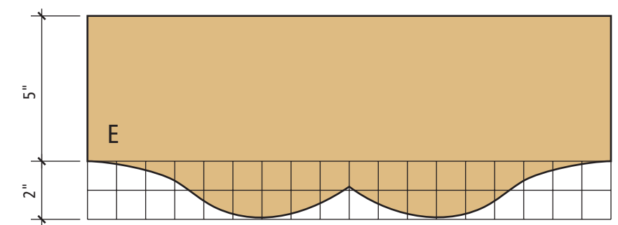
Bottom rail
