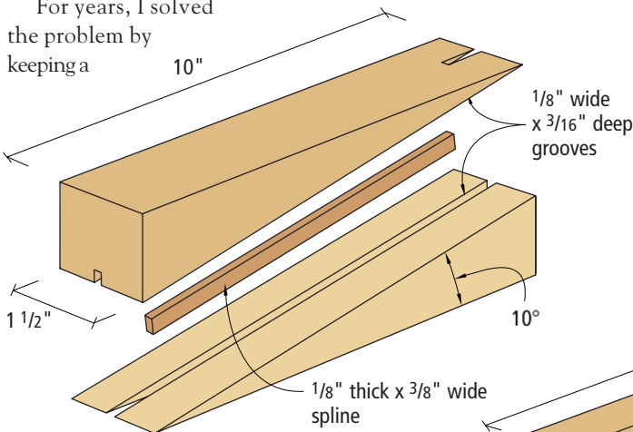
Grooved Wedges
