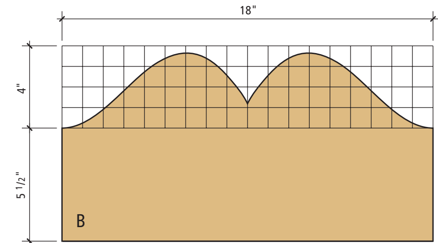
Top rail
