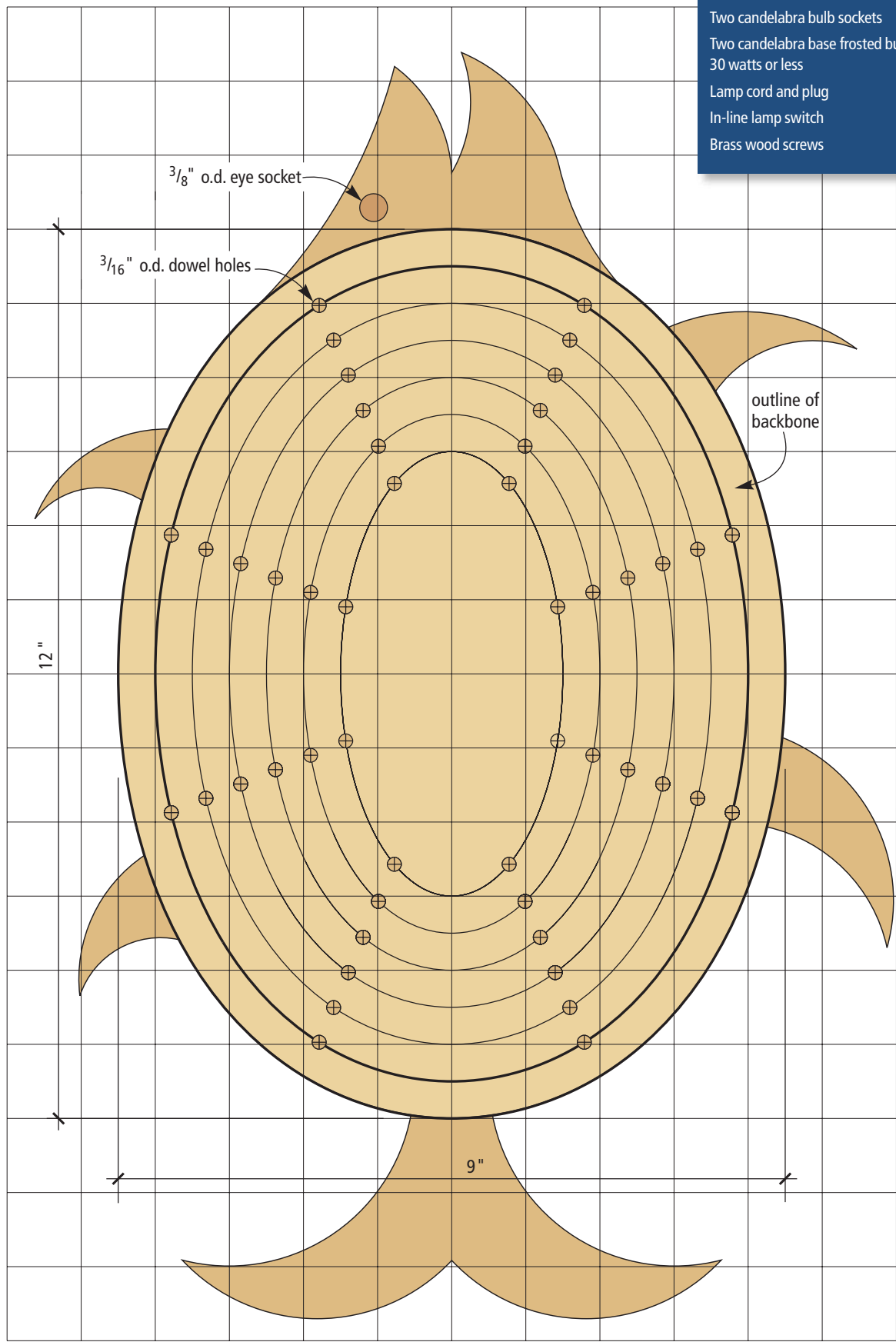
Half-scale drawing; enlarge 200 percent for full-size
