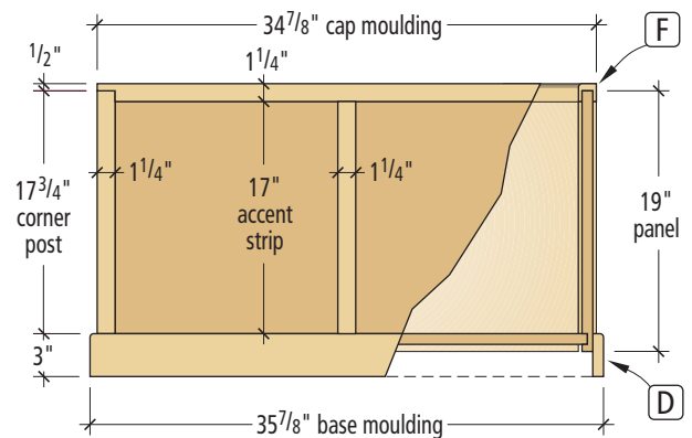
Elevation - section
