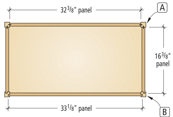
Plan - lid removed
