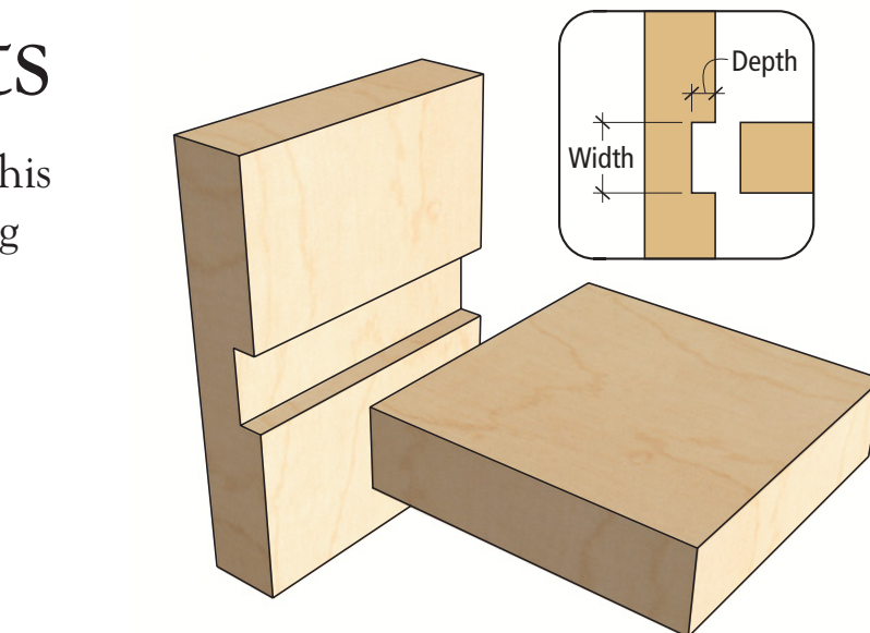
Through dado
