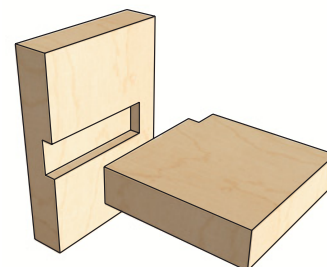
Stopped dado
