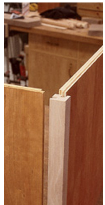
Tongue-and-groove joint
