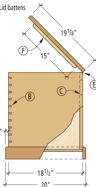
Profile - section
