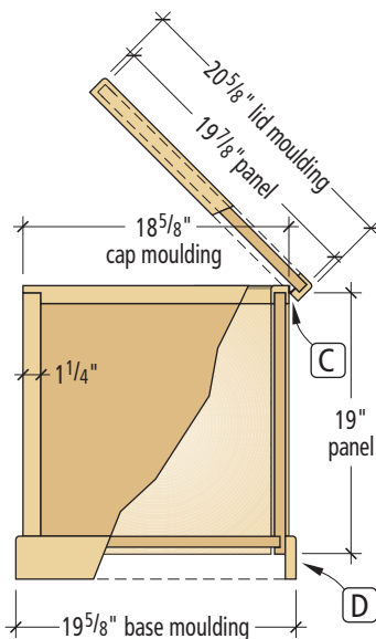
Profile - section
