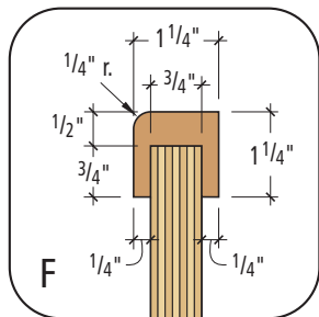
Cap moulding
