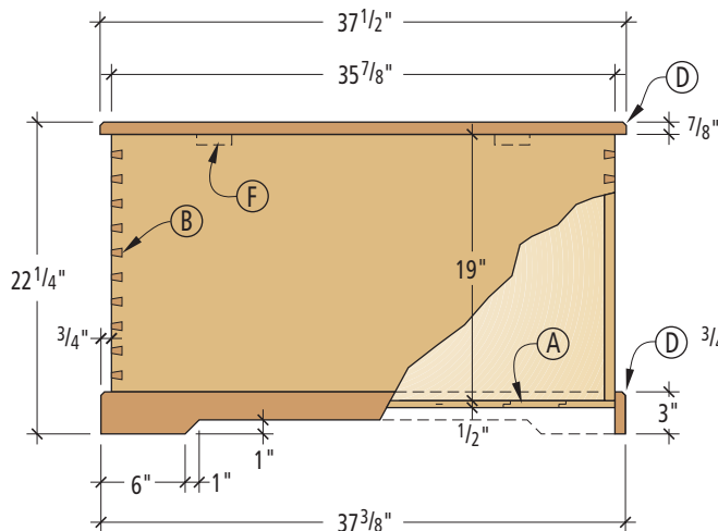
Elevation - section
